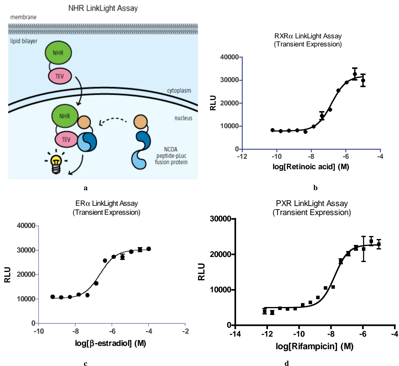
Fig. (2). NHR LinkLight Assay. a , A schematic drawing of NHR-TEV and NCOA1-pLuc interaction LinkLight assay. b , U-2 OS cells stably expressing NCOA1-pLuc and transiently expressing RXR \alpha -TEV genes showed dose-response curve in response to the ligand retinoic acid. c , U-2 OS cells stably expressing NCOA1-pLuc and transiently expressing ER \alpha -TEV genes showed dose-response curve in response to the ligand \beta -estradiol. d , U-2 OS cells stably expressing NCOA1-pLuc and transiently expressing PXR-TEV genes showed dose-response curves in response to the ligand rifampicin. Data points are represented as mean \pm SD from n=3 . EC 50 values were derived from non-linear regression with the best-fit equation.
