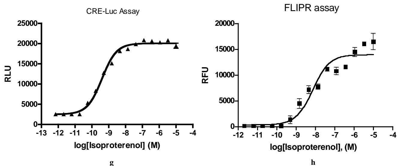
Fig. (1). GPCR LinkLight assay. a. The design of LinkLight assay technology. b. A schematic draw of GPCR-TEV and \beta -arrestin-pLuc interaction LinkLight assay. Molecules trigger the interaction of GPCR-TEV fusion protein and \beta -arrestin-pLuc fusion protein, resulting in the cleavage of the inactive permuted luciferase and reconstitution of an active luciferase. c. GPCR LinkLight assay with two different designs. ADRB2-TEV and Arr2-pLuc plasmids or Arr2-TEV and ADRB2-pLuc-V plasmids were co-expressed transiently in HEK293 cells to produce ligand-induced luciferase signals. d. Dose response curves of ligands in HEK293 cells stably expressing ADRB2-TEV and Arr2-pLuc fusion proteins. e. HEK293 cells stably expressing V2R-TEV and Arr2-pLuc-V fusion proteins and their response to the V2 agonist, Arg8-vasopressin. f. cAMP assay using HEK293 cells transiently expressing ADRB2-TEV fusion gene in response to agonists, partial agonists, and antagonists. g. Cre-Luc assay using CHO cells stably expressing CRE-Luc and transiently expressing ADRB2-TEV genes in response to isoproterenol. h. FLIPR assay using HEK293 cells stably expressing Ga16 and transiently expressing ADRB2-TEV genes in response to isoproterenol. All curves were generated by using GraphPad Prism 5 software. Data points are represented as mean \pm SD from n=3 . EC_{50} values were derived from non-linear regression with the best-fit equation.
